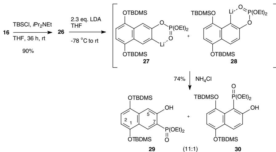
Scheme 4. Rearrangement of an aryl phosphate.
